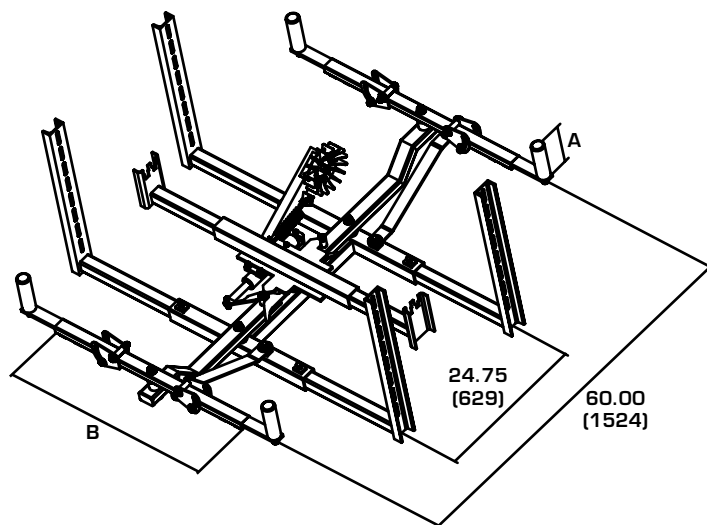
Lower Unit
